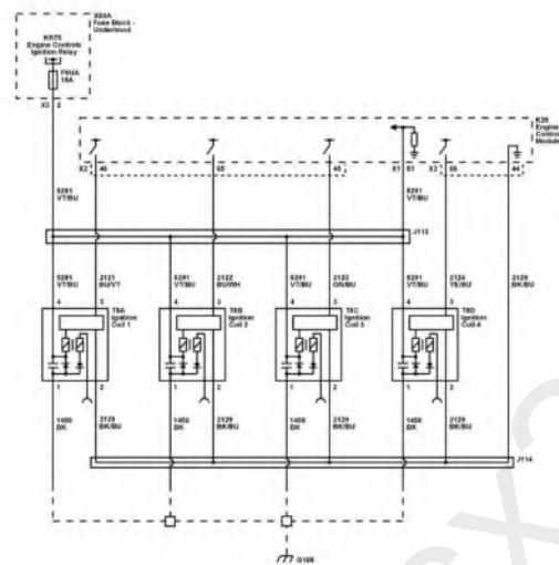
Ignition Controls - Ignition Sensors, and Camshaft Actuators
